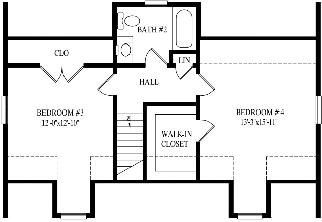
Proposed Second Floor – 674 sq. ft.
