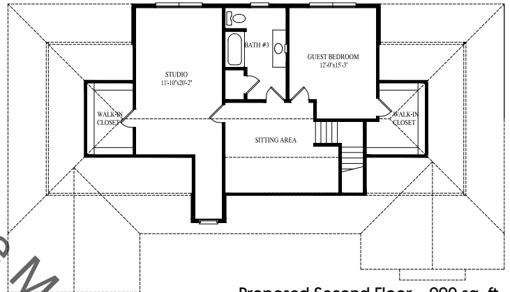
Proposed Second Floor – 990 sq. ft.
