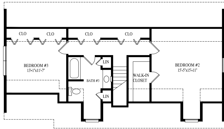
Proposed Second Floor – 814 sq. ft.
