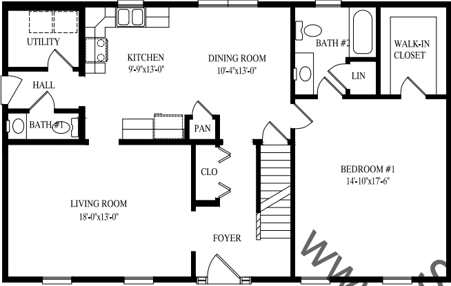
Huntington I 27' 6" x 41' Cape 1210 sq. ft. first floor
