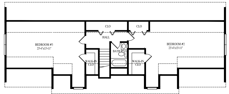
Proposed Second Floor – 875 sq. ft. w/garage option – 1079 sq. ft.
